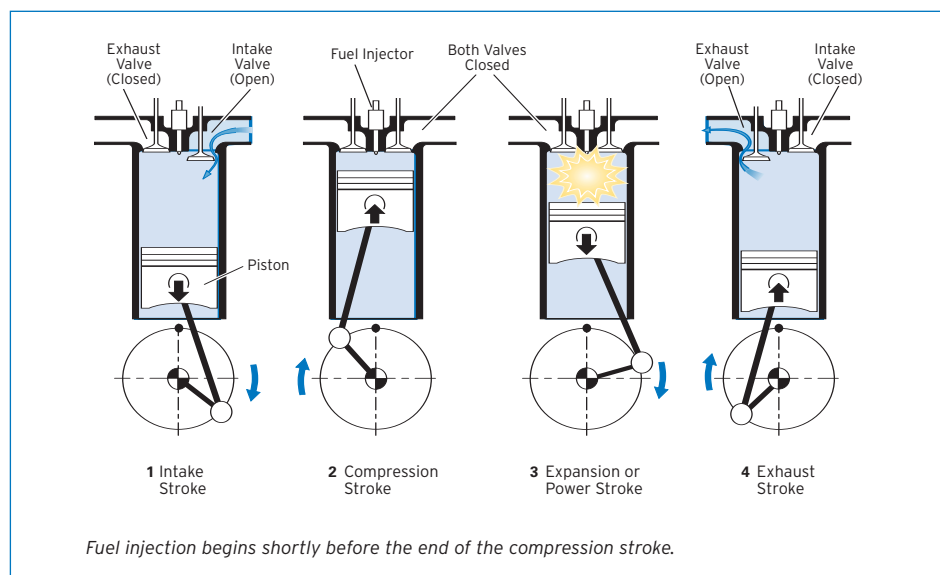
Figure 6.1 Four-Stroke Cycle
