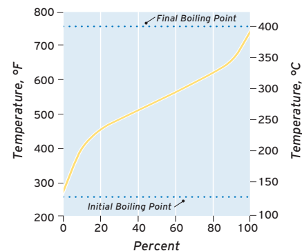
Figure 4.3 Typical Distillation Profile - No. 2-D Diesel Fuel
