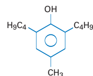
2,6-Di- t -butyl-4-methyl phenol
